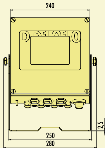
DD1010i desk-stand version
