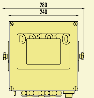
DD1010i wall-mounted version
